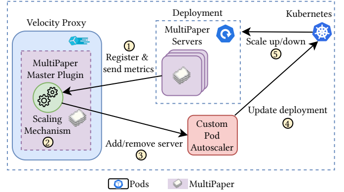
Fig. 2: Dynamic scaling process.
