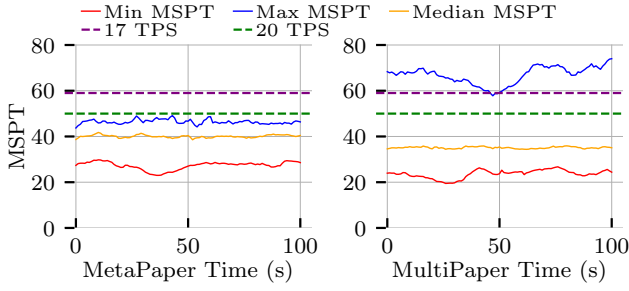
(a) MetaPaper achieves MSPT under 50 ms with 800 users, enabling gameplay at 20 TPS. MultiPaper fails to keep TPS at 20 for all servers in this scenario.
