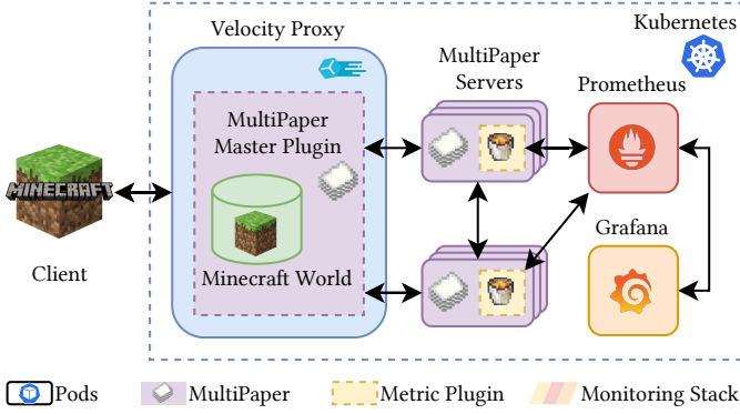
Fig. 1: MetaPaper architecture.
