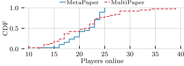
(b) Player distribution across servers is more balanced in MetaPaper, contributing to better user experience.
