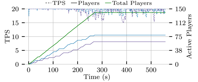
Fig. 5: MetaPaper - TPS and Players per Server (2 servers, up to 140 players): Improved load balancing distributes players more evenly across servers, achieving higher TPS stability.
